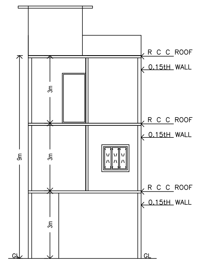
SECTION @ X-X
